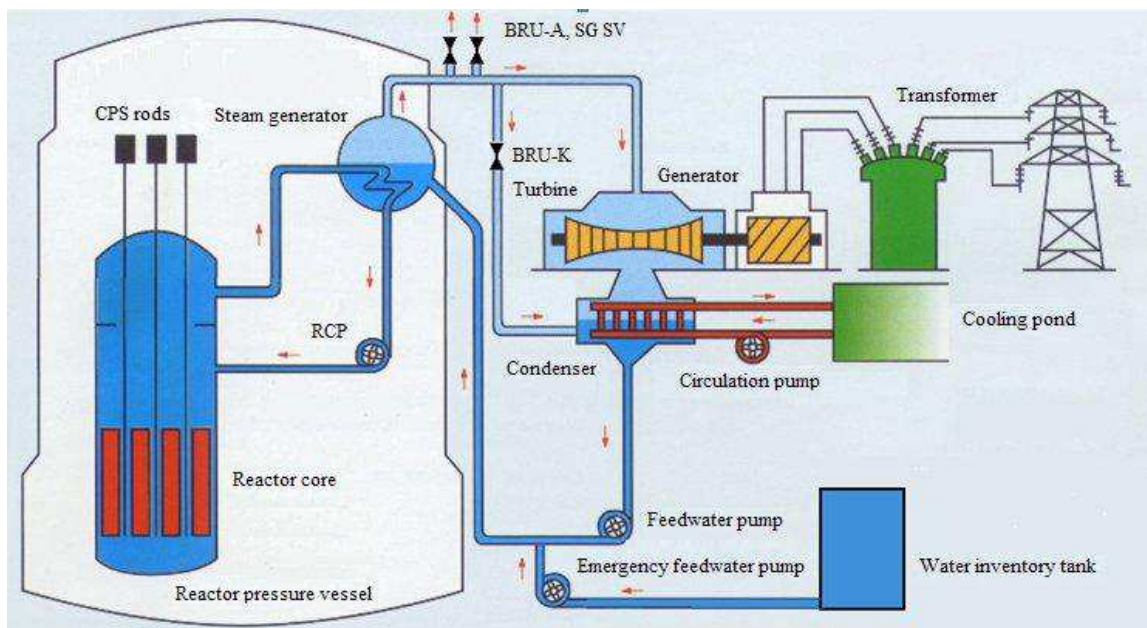
Fig. 2.4. Process diagram of heat removal to ultimate heat sink for NPP with VVER units (design without cooling towers)
