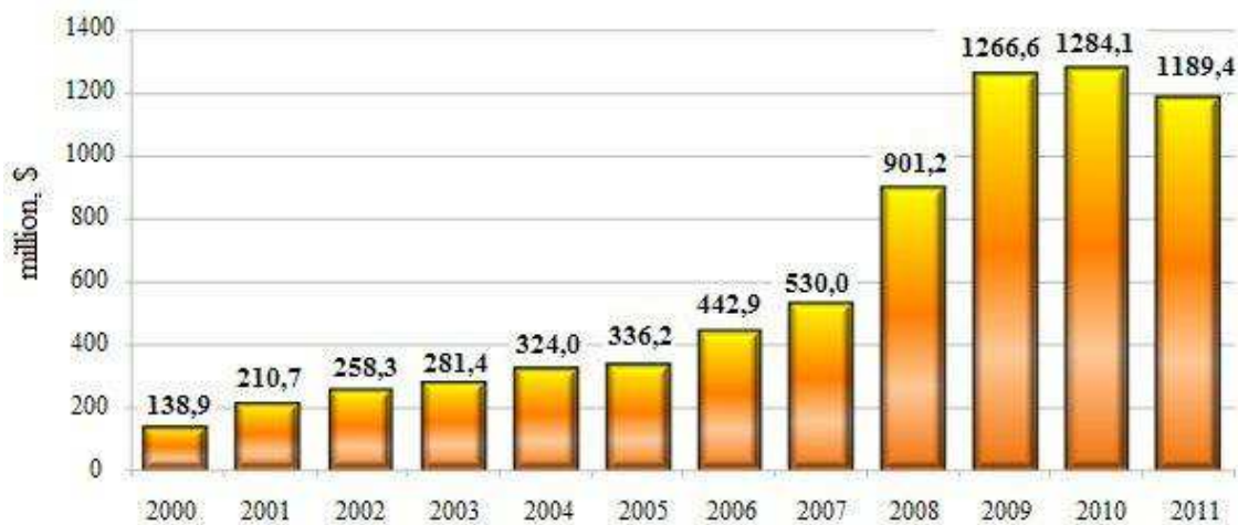
Fig. I.2. Funding of the retrofit activities for the NPPs in operation in Russia
