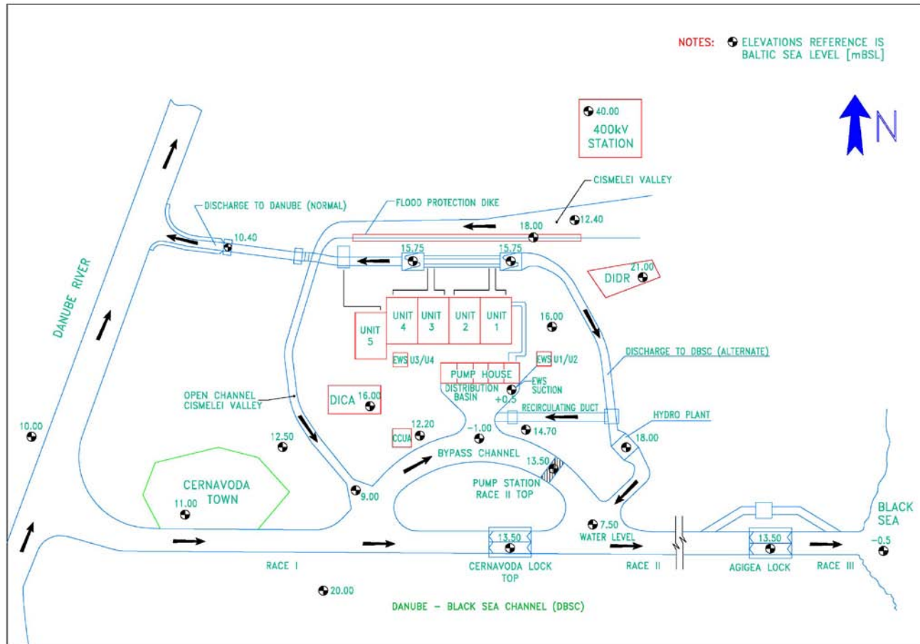
Fig. 1.2 Cernavoda NPP site elevations
