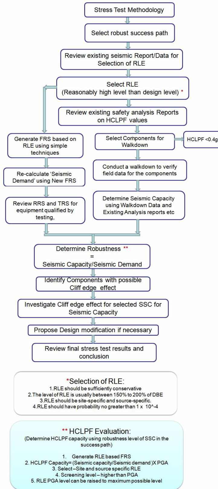
Fig. 1.1. Seismic Margin Evaluation Methodology
