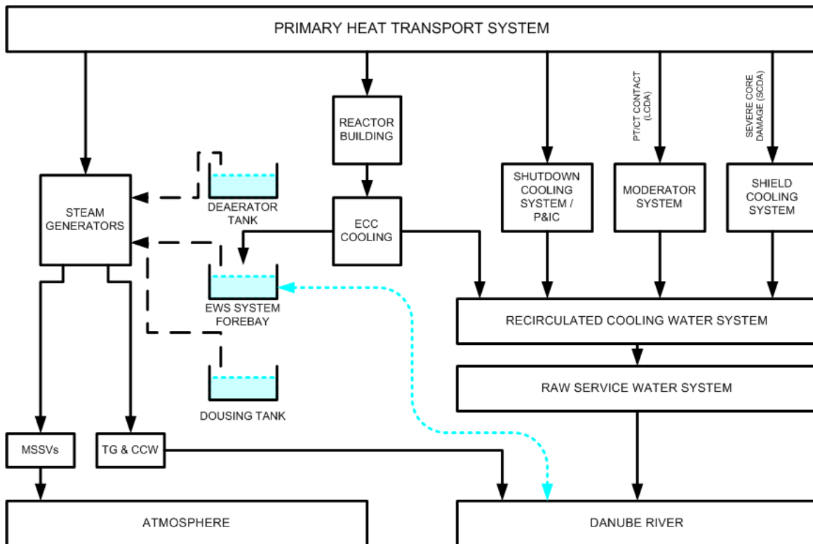
Figure 2.2 Schematic of Core Heat Sinks in CANDU-6
