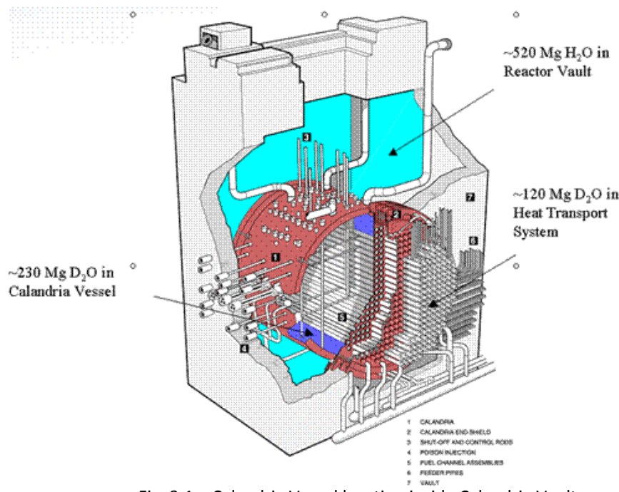
Fig. 3.1 – Calandria Vessel location inside Calandria Vault
