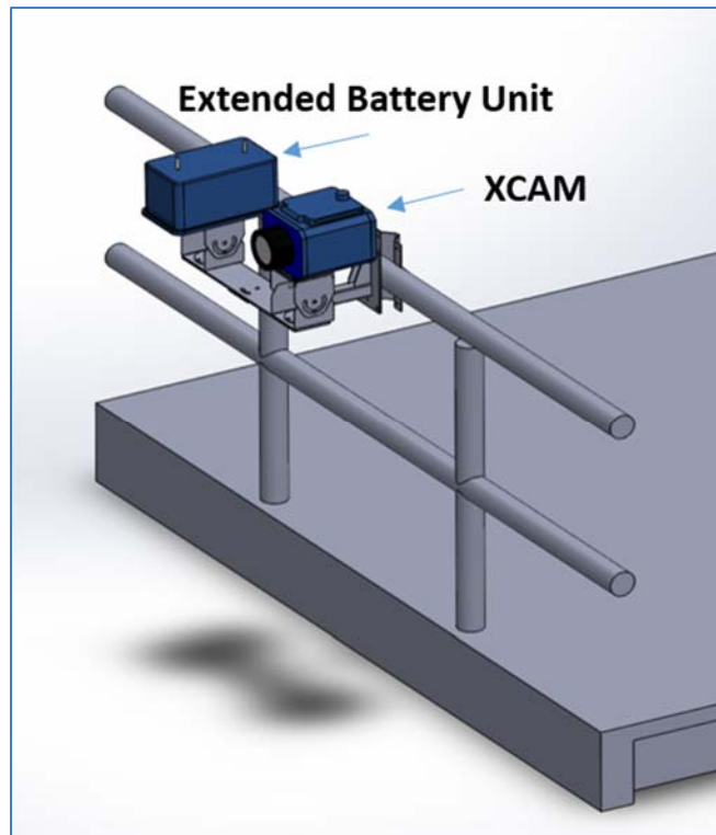
Figure 57: XPCAM Deployment Configuration
