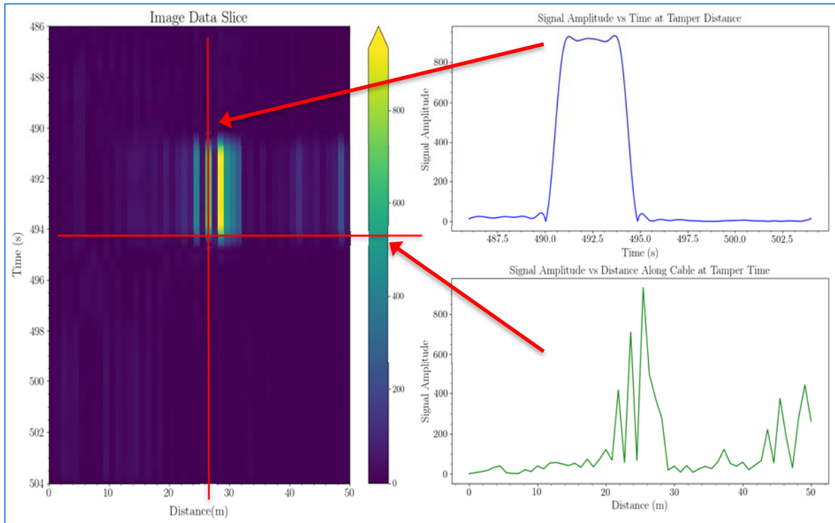
Figure 69: TDR (Time Domain Reflectometry) technique showing typical tamper along the detector cable at about 25 m from the cabinet
