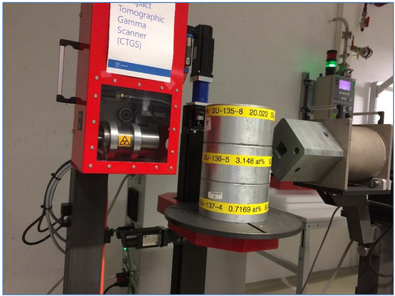
Figure 49: Compact Tomographic Gamma Scanner (CTGS)
