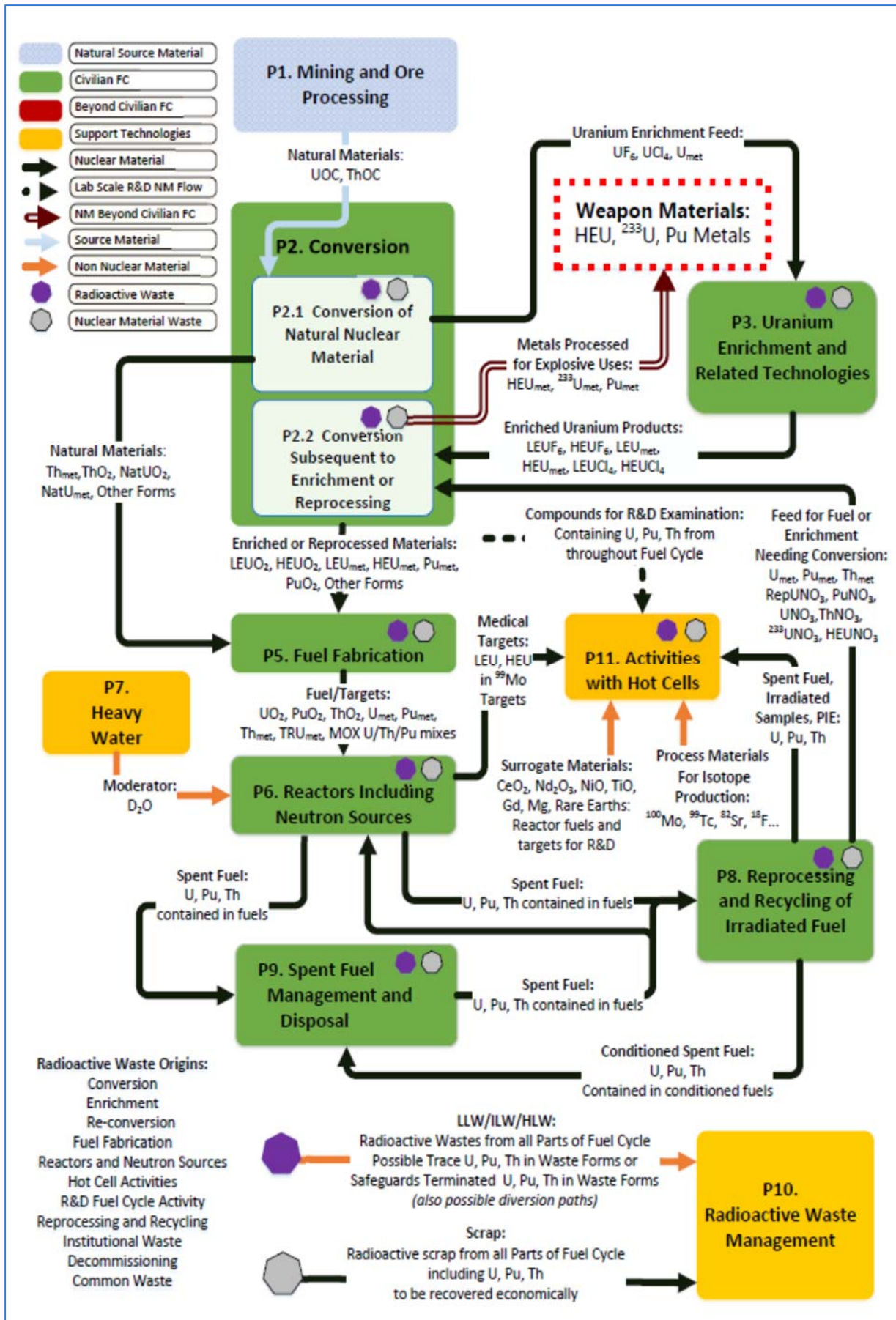
Figure 18: Physical Model flow diagram
