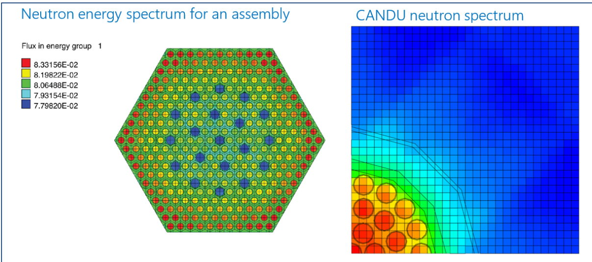
Figure 33: Reactor modelling examples for determining fuel burn-up for comparison to ES analytical results.
