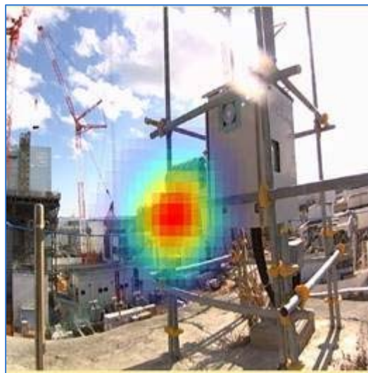
Figure 66: Output of the gamma imaging system in a field test
