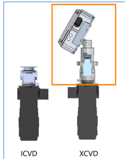
Figure 65: Comparison of the architecture of ICVD and XCVD
