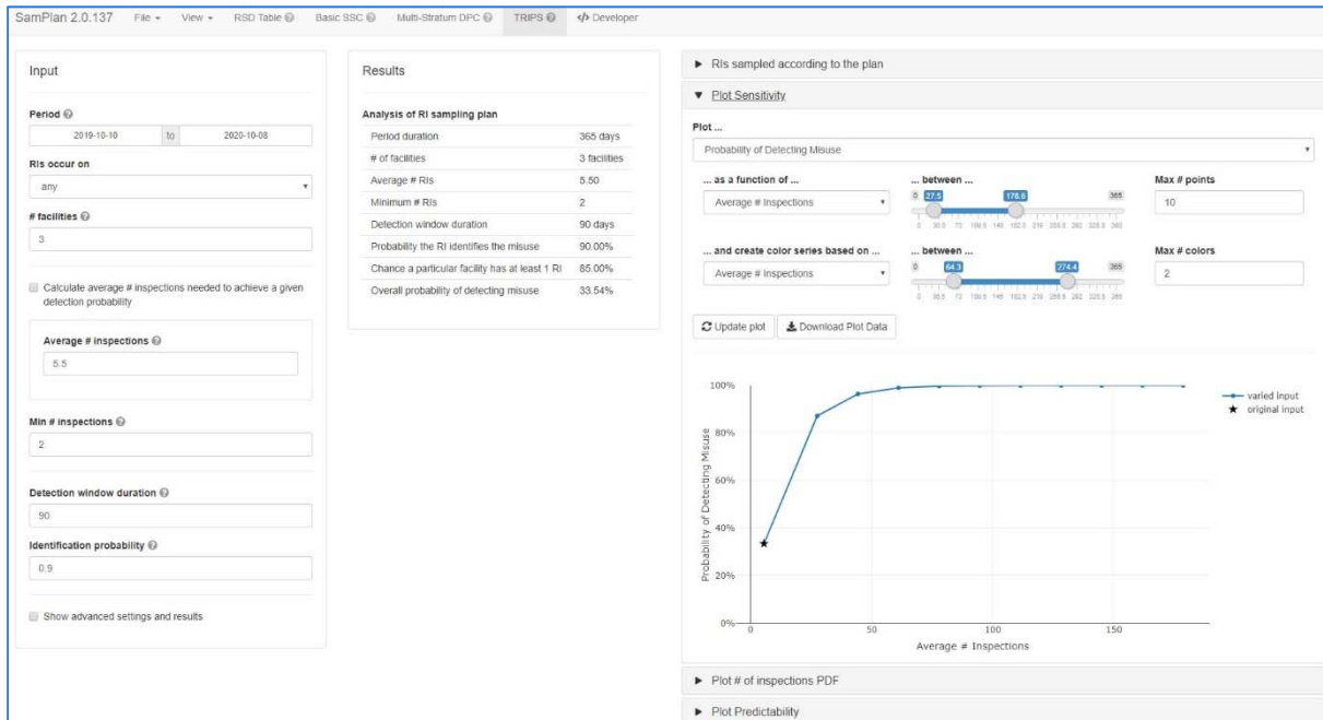
Figure 35: Random Inspection Calculation Tool
