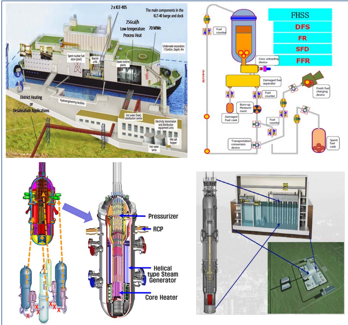
Figure 16: New types of Small Modular Reactors (SMRs).
