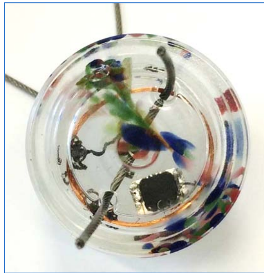
Figure 53: Concept of New Passive Seal with high-security RFID
