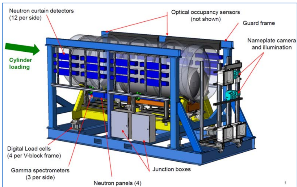
Figure 70: Drawing of the UCVS system
