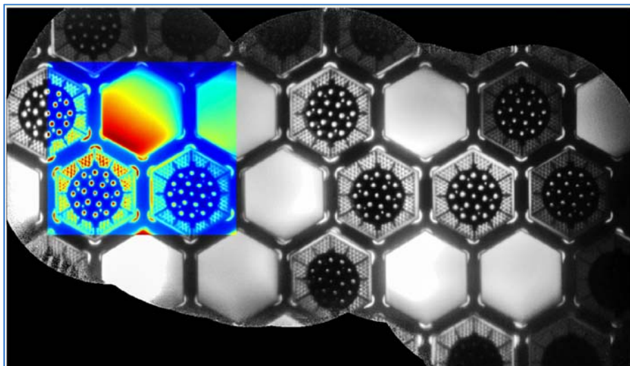
Figure 66: Output of the gamma imaging system in a field test
