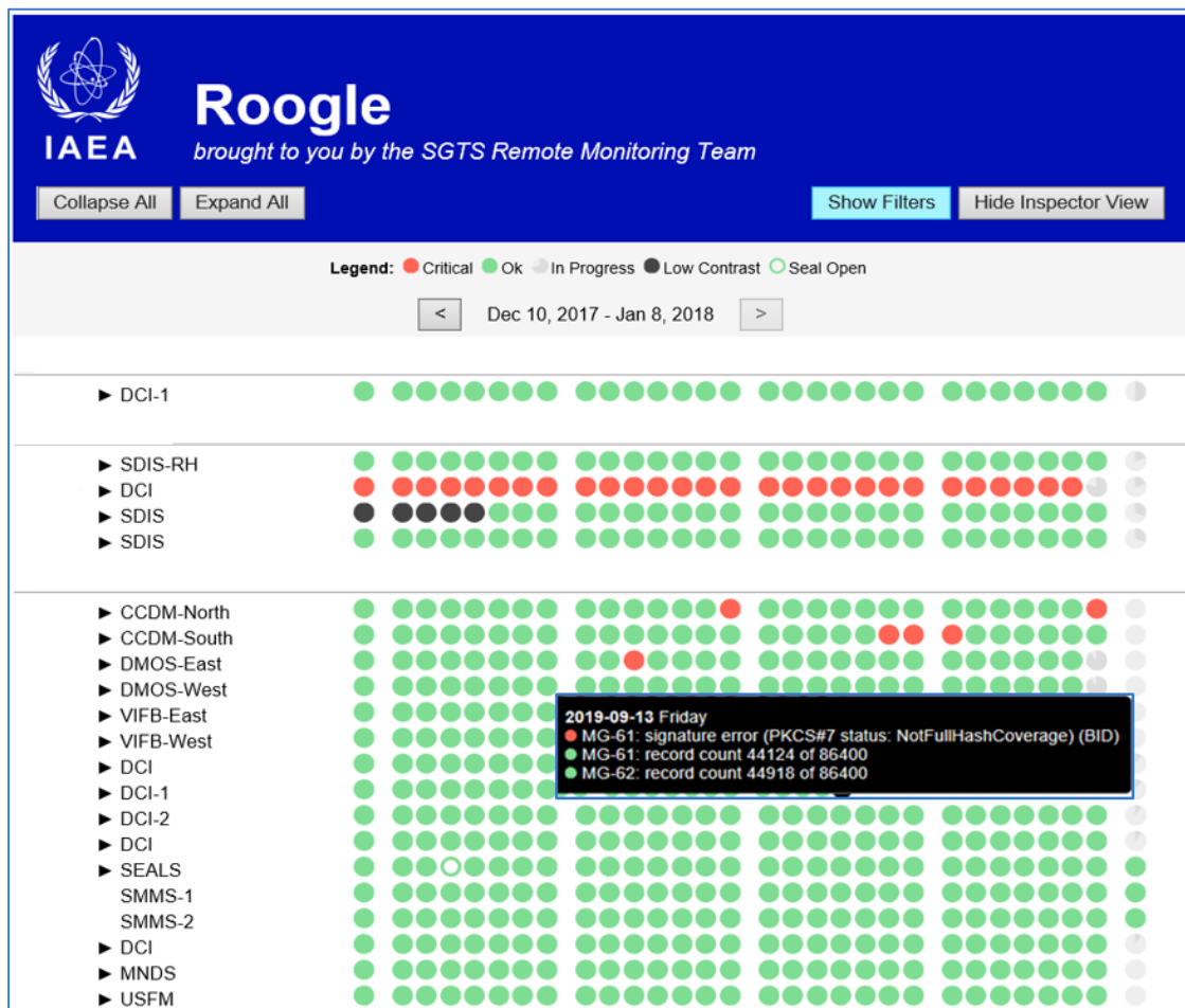
Figure 74: Screenshot of Roogle2 with 'status of health' information
