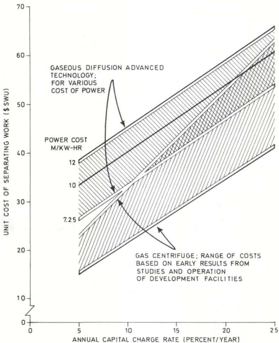
Figure 6. Comparison of technologies 8.75 million SWU/year plant at a new site.
